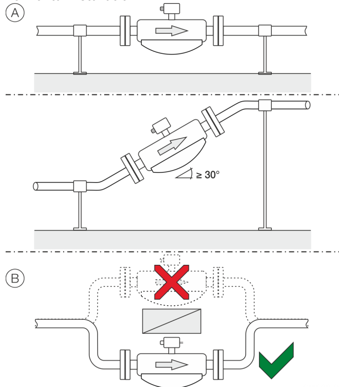
Figure 5: Horizontal installation
