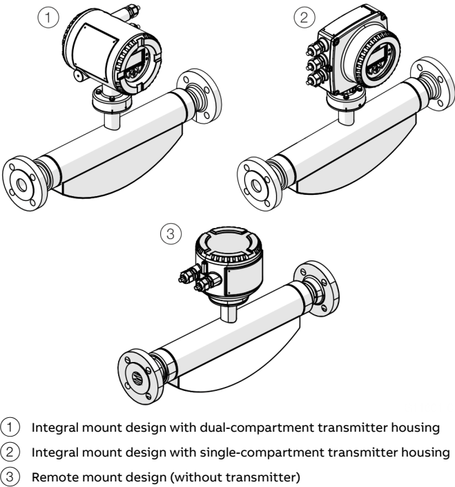
Figure 10: Sensor FCB4xx / FCH4xx
