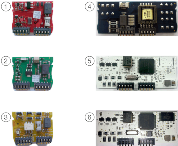
Figure 21: Plug-in cards
