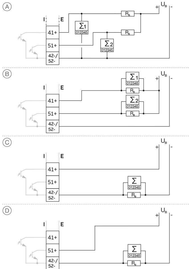
Figure 39: Connection versions digital output 41 / 42 and 51 / 52
