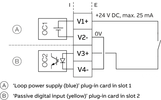
Figure 38: Active digital output V3 / V4 (example)
