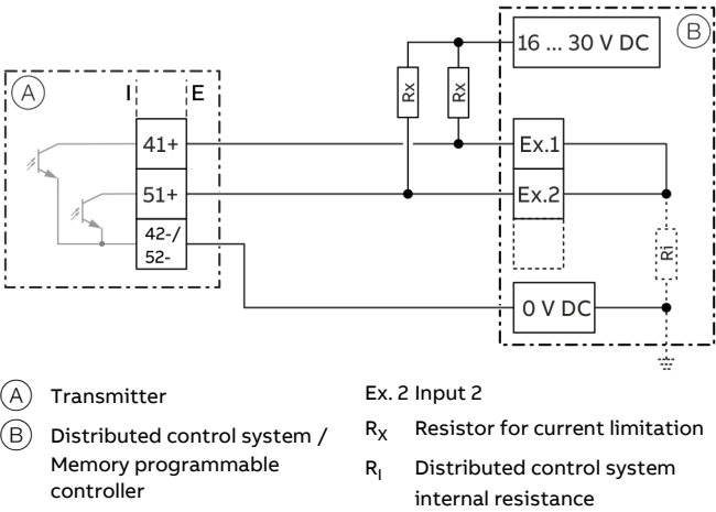
Figure 36: Digital output 41 / 42 on distributed control system (example)
