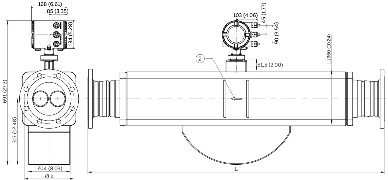
Figure 4: Integral mount design with dual-compartment transmitter housing
