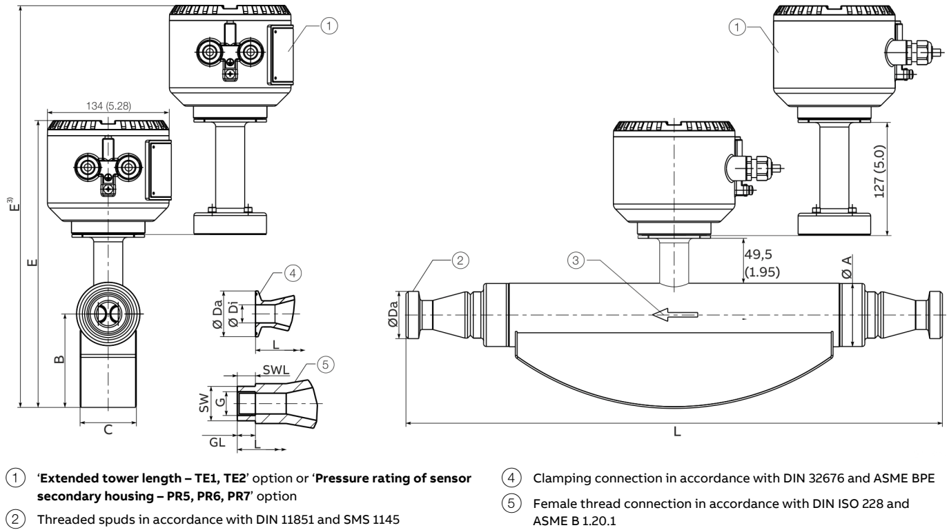
Figure 11: Remote mount design
