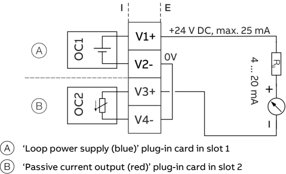
Figure 37: Active current output V3 / V4 (example)
