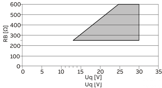
Permissible source voltage U_q for passive outputs in relation to load resistance R_B where I_{max} = 22\text{ mA} . = Permissible range
