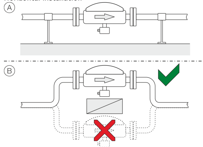
Figure 6: Horizontal installation
