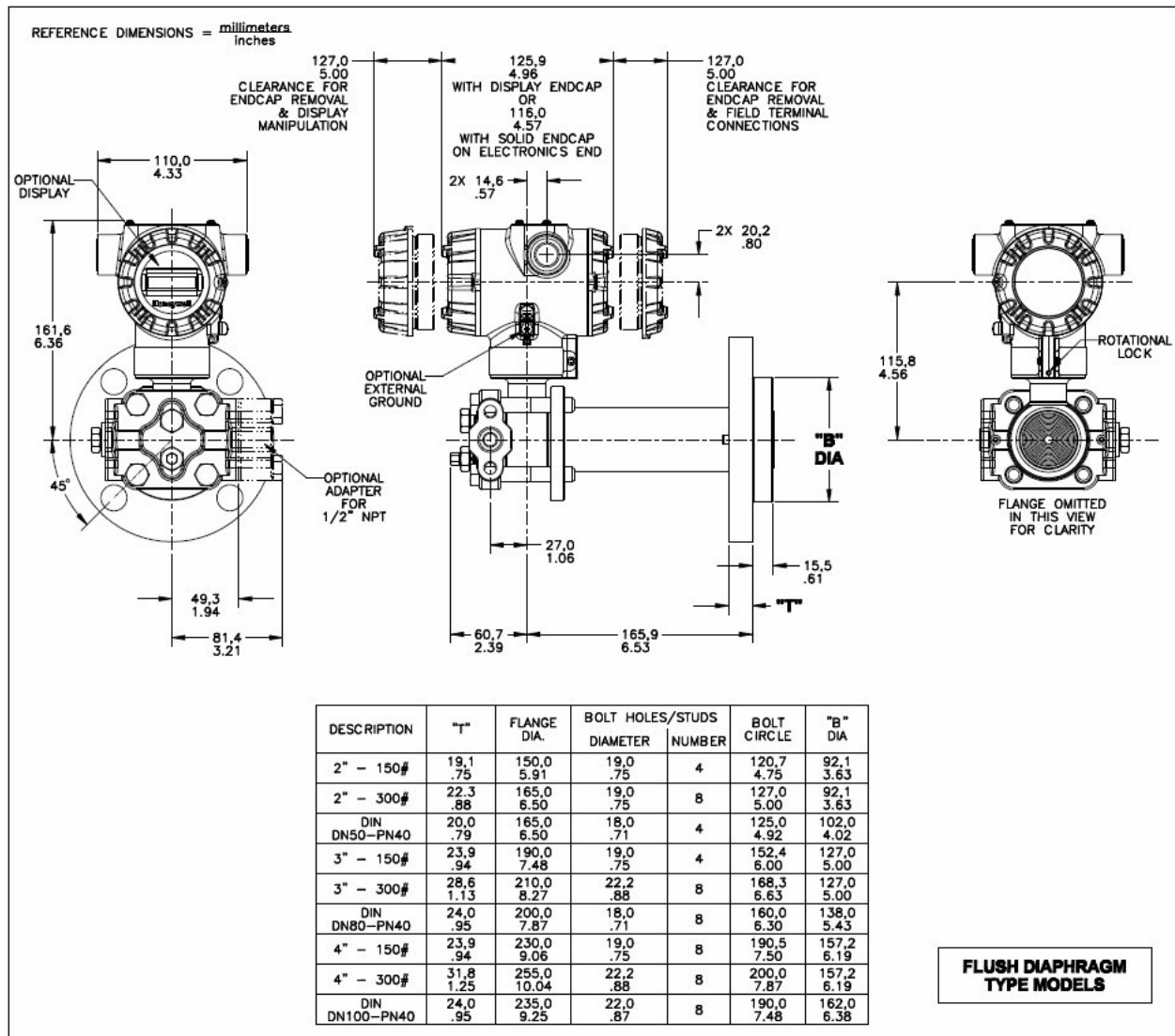
Figure 4– Typical mounting dimensions for flush diaphragm type models STF828 and STF832.
